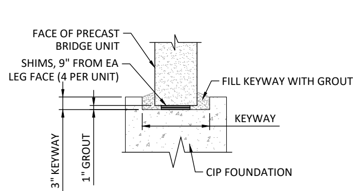
UNIT GROUT DETAIL NOT TO SCALE
