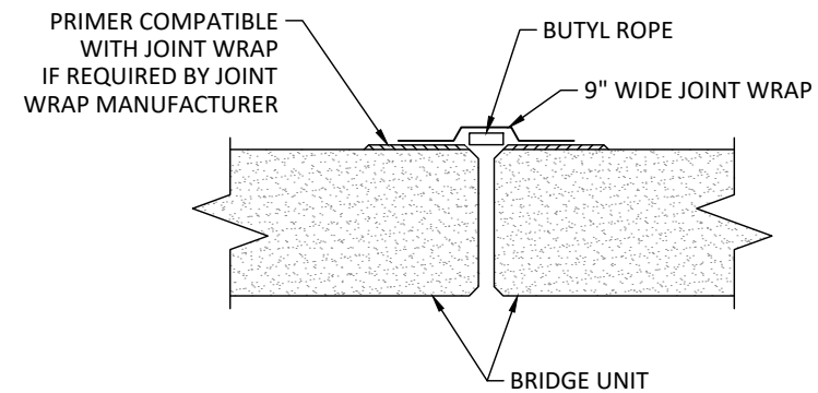
JOINT SEAL DETAIL NOT TO SCALE
